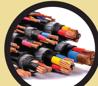
PVC/SWA/PVC (P/S/P) Armoured Cables
